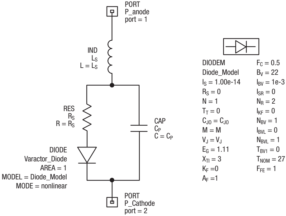
Figure 3. SPICE Model
